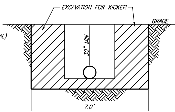
EXCAVATION SECTION A-A NO SCALE
