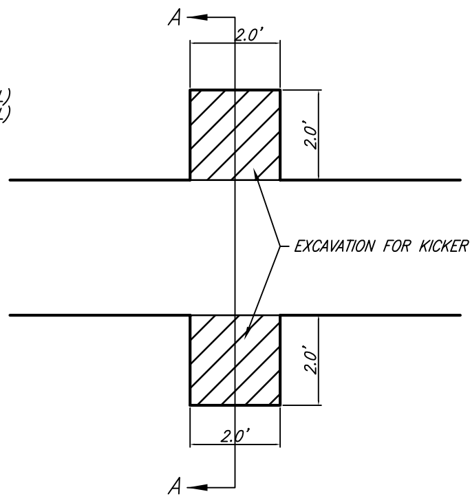
EXCAVATION PLAN NO SCALE
