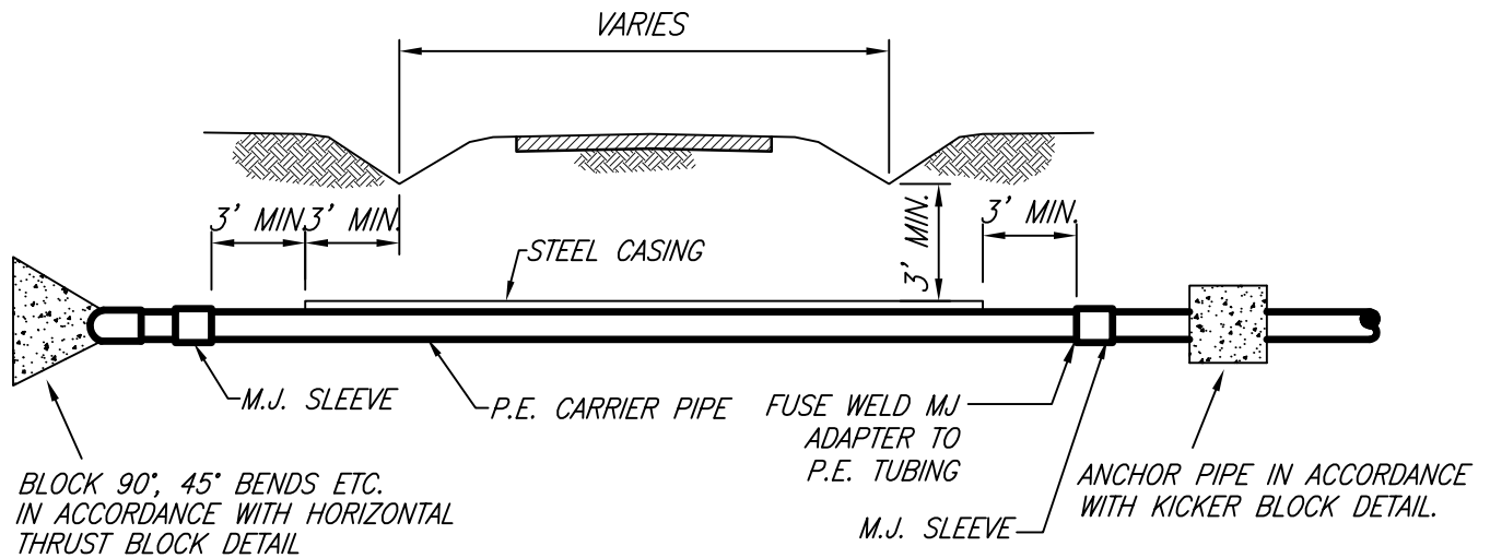
BORE DETAIL W/ THRUST BLOCK & KICKER BLOCK
