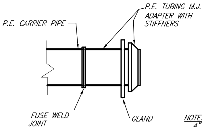
ADAPTER DETAIL
